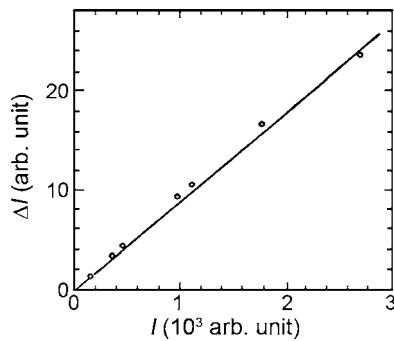
Fig. 3.24 The linear curve of \Delta I vs. I for sample 3 ( x = 0.34 ) under the condition of a fixed pump beam power I_{\text{pumb}} and temperature T = 300 K ( Q_p = 5.4 \times 10^{18}/\text{s cm}^2 , \sigma(E) = 1.5 \times 10^{-15} \text{ cm}^2 , with slope \Delta I/I = 8.8 \times 10^{-3} , the probe beam is a \text{CO}_2 laser ( \lambda = 10.6 \mu\text{m} ) and the pump beam is a He-Ne laser ( 0.6328 \mu\text{m} ))
