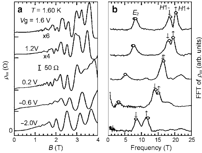
Fig. 5.31 The variation of SdH oscillations and its FFT resulting variation with gate voltage for a symmetric HgTe quantum well
