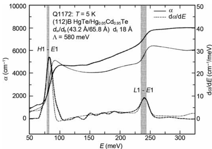
Fig. 5.24 The absorption spectrum of \text{HgTe}/\text{Hg}_{1-x}\text{Cd}_x\text{Te} superlattice at T = 5 K. The measured absorption coefficient and its differential results are shown by a thick solid curve and dashed curve, the calculated ones are shown by a thinner solid curve and a dashed curve
