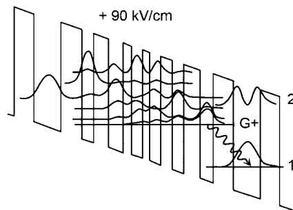
Fig. 6.67 Conduction band diagram of two active regions with the intermediate injector region of a diagonal transition active region QC laser under a positive applied electric field of 90\ \text{kV}/\text{cm} approximately corresponding to laser threshold. The layer thicknesses in nanometres are from left to right starting from the first injection barrier: 3.5/4.8/3.5/2.4/2.5/2.6/1.5/2.2/1.0/2.2/1.9/2.2/2.9/2.2/3.5/4.8/3.5. The \text{In}_{0.52}\text{Al}_{0.48}\text{As} layers (energy barriers) are in bold symbols alternated with the \text{In}_{0.53}\text{Ga}_{0.47}\text{As} wells. The underlined layers are doped to n = 4 \times 10^{17}\ \text{cm}^{-3} ; italic style indicates the injector region. The absolute value squared of the wavefunctions in the active and injector regions are shown. The wavy arrow indicates the laser transition G_+ \rightarrow \mathbf{1}
