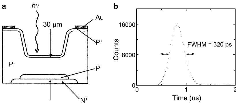
Fig. 6.93 (a) A schematic of a reach-through SPADs cross section. (b) The time resolution of the device at room temperature for a spot of light located in the center of the device with a diameter 50\text{ }\mu\text{m} . The photodiode was operated in a gated mode at 40 V excess bias, with an active quenching circuit (Ghioni and Ripamonti 1991)
