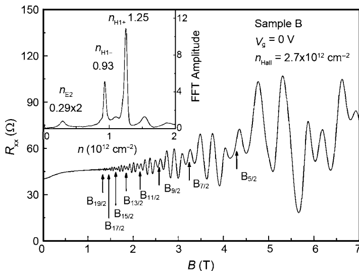
Fig. 5.36 The measured SdH oscillations R_{xx} of sample B. The arrows show the node positions of the beat pattern. The insert shows the FFT results
