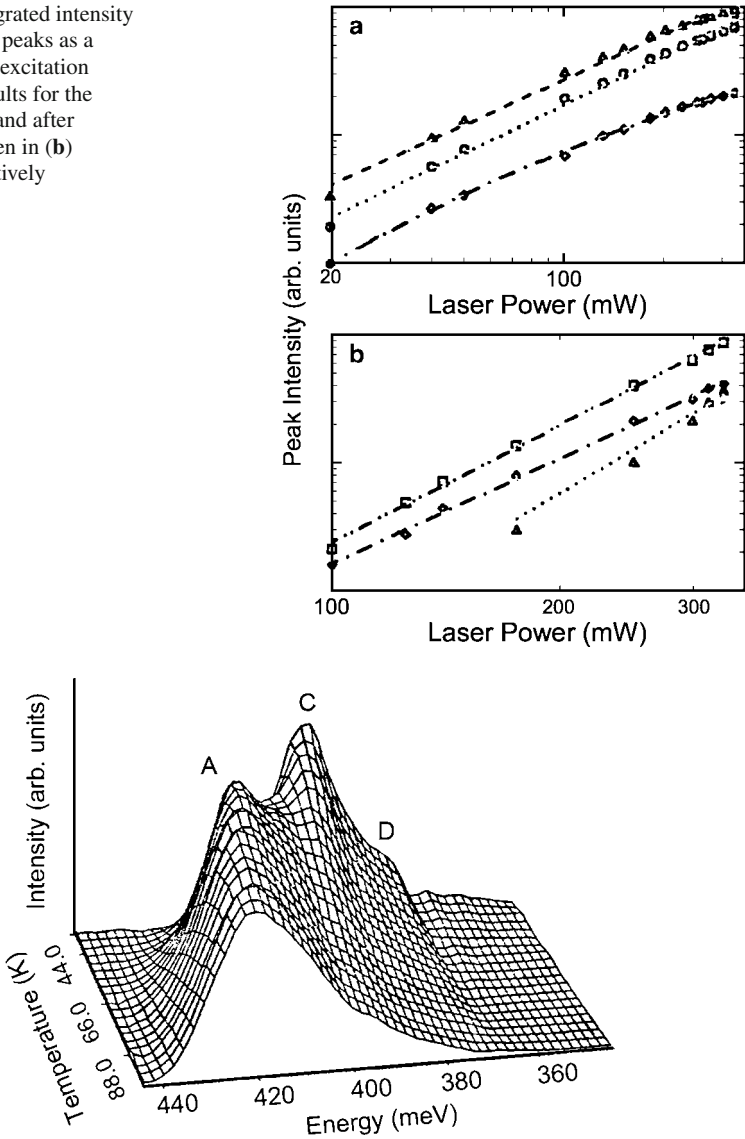
Fig. 2.85 Temperature-dependent PL spectra for samples after etching
