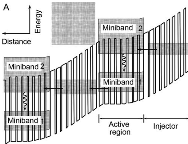
Fig. 6.65 A schematic conduction-band structure of the original InGaAs/InAlAs SL-QC laser. The shaded regions indicate the minibands. Laser action, denoted by the wavy arrows , takes place across the first minigap 2 \rightarrow 1 . The applied electric field is screened from the flat SLs through extrinsic electrons
