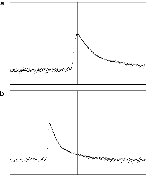
Fig. 2.23 The positron annihilation spectra technology (PAT) spectrum of a p-type HgCdTe sample (a) and that for the same sample three months later (b)
