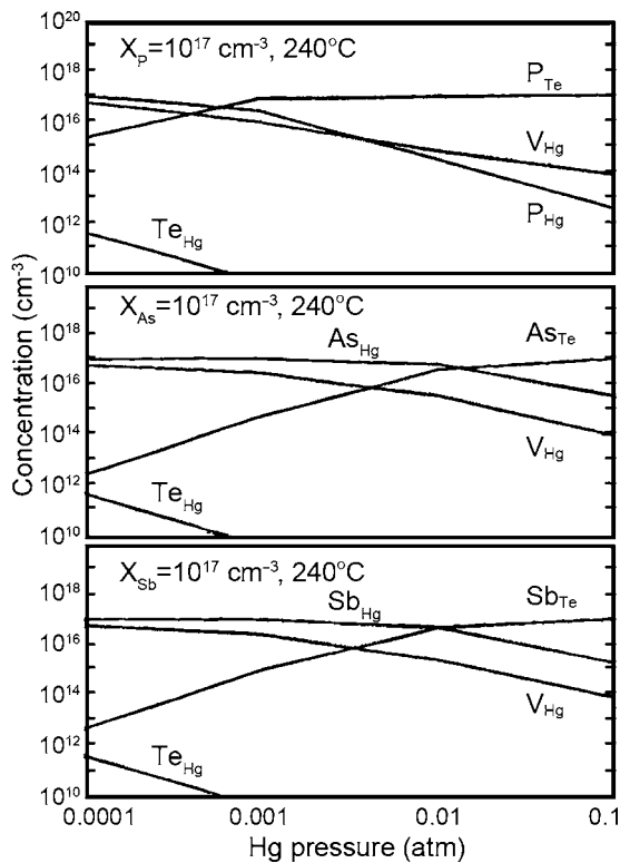
Fig. 2.11 P, As and Sb defect concentrations on the anion and cation sublattice sites as a function of Hg partial pressure for HgCdTe samples equilibrated at 240° C. The Hg vacancy and Te antisite concentrations are also shown
