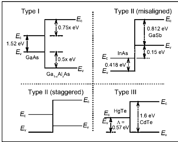
Fig. 5.9 Band edge alignment of three types of heterostructures
