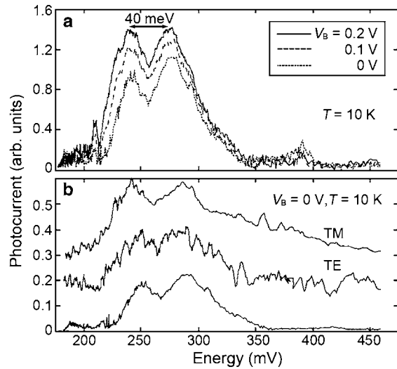
Fig. 6.54 A normal incidence photocurrent spectra of an In(Ga)As/InGaAs QD detector: (a) measured at different bias voltages, (b) the polarization-dependent photocurrent for a waveguide geometry (Chu et al. 1999b)
