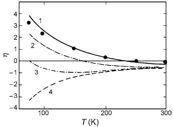
Fig. 2.37 Fermi energy levels of a series of HgCdTe samples ( x = 0.194 ) with different donor concentrations. curve 1: N_D = 2.2 \times 10^{16} \text{ cm}^{-3} , curve 2: N_D = 1 \times 10^{16} \text{ cm}^{-3} , curve 3: N_D = 2.26 \times 10^{15} \text{ cm}^{-3} , and curve 4: intrinsic condition
