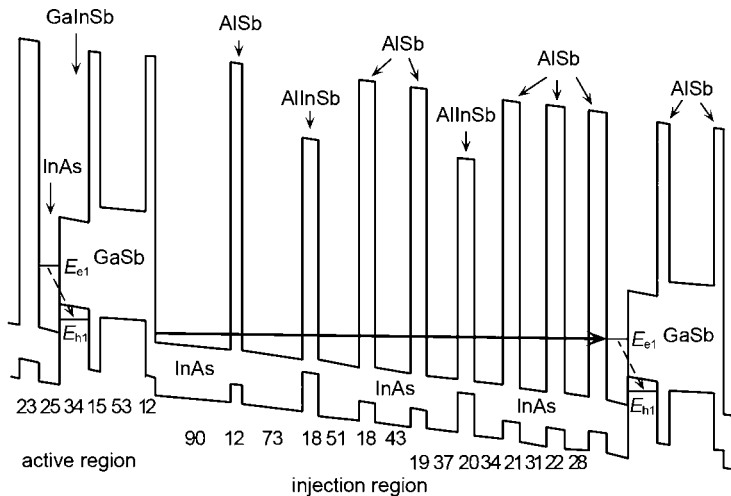
Fig. 6.78 A schematic electronic band structure for a type-II InAs/GaInSb/Al(In)Sb QW interband transition QCL. The numbers near the bottom of the figure indicate layer thicknesses (in Å). The compositions of the ternary alloys are \text{Ga}_{0.7}\text{In}_{0.3}\text{Sb} and \text{Al}_{0.7}\text{In}_{0.3}\text{Sb} , respectively (Yang 2000)
