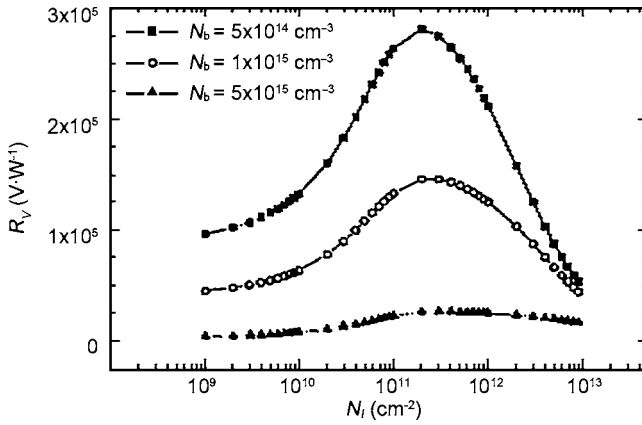
Fig. 3.55 Relations between voltage responsivity R_v of devices that have different doping densities N_b , and the density of surface fixed electric charge N_t
