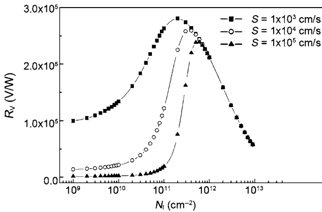
Fig. 4.65 The voltage responsivity R_v for devices with different surface recombination velocities S_0 as a function of the concentration of surface bound charges N_l . The values of other parameters are N_b = 5 \times 10^{14} \text{ cm}^{-3} and \tau_b = 1 \mu\text{s}
