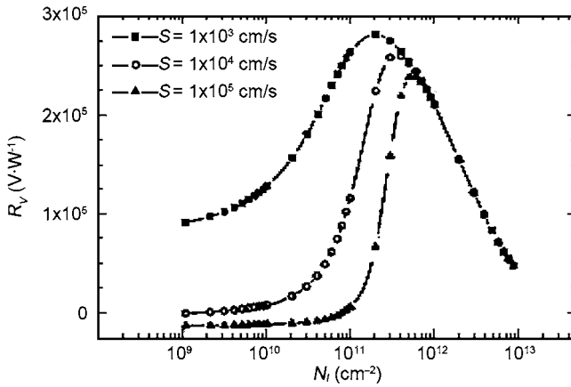
Fig. 3.56 Relations between voltage responsivity R_v of devices that have different surface recombination rates S_0 , and the density of fixed electric surface charge N_t
