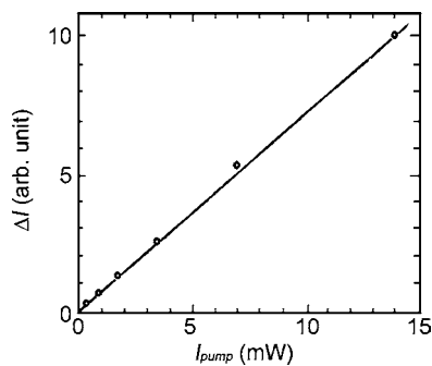
Fig. 3.25 The linear curve of \Delta I vs. I_{\text{pumb}} for sample No. 3 ( x = 0.34 ) under the condition of fixed-probe beam power I_{\text{probe}} and temperature T = 300 K ( \lambda_{\text{probe}} = 10.6 \mu\text{m} , \lambda_{\text{pump}} = 0.6328 \mu\text{m} ) and in this case the result is the same as that obtained in Fig. 3.24 ( \tau = 3.6 \times 10^{-7} \text{ s} )
