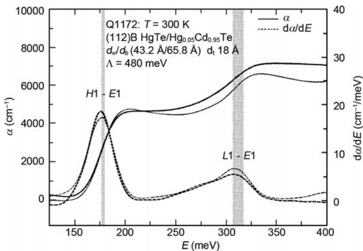
Fig. 5.25 The absorption spectrum of a \text{HgTe}/\text{Hg}_{1-x}\text{Cd}_x\text{Te} superlattice at T = 300 K
