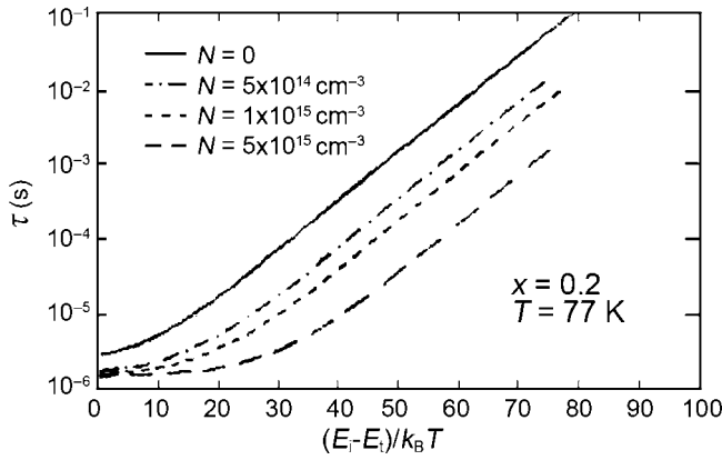
Fig. 3.5 The relation between the R-S recombination lifetime and (E_i - E_t)/k_B T
